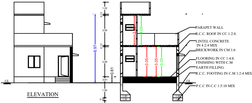
SECTION HK'
