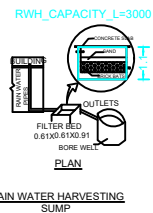
RAIN WATER HARVESTING SUMP
