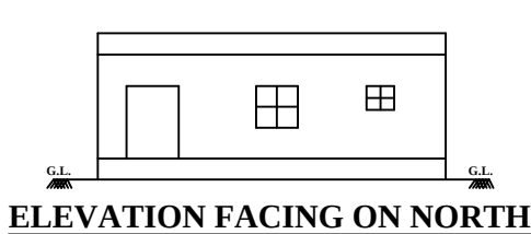
ELEVATION FACING ON NORTH
