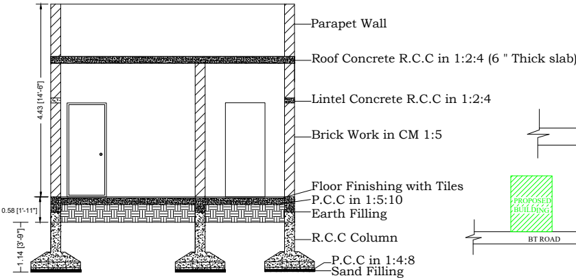
SECTION X-X
