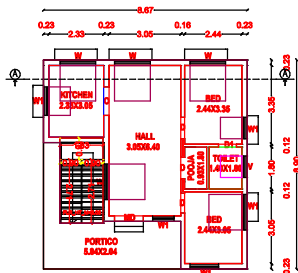
PROPOSED GF.PLAN
