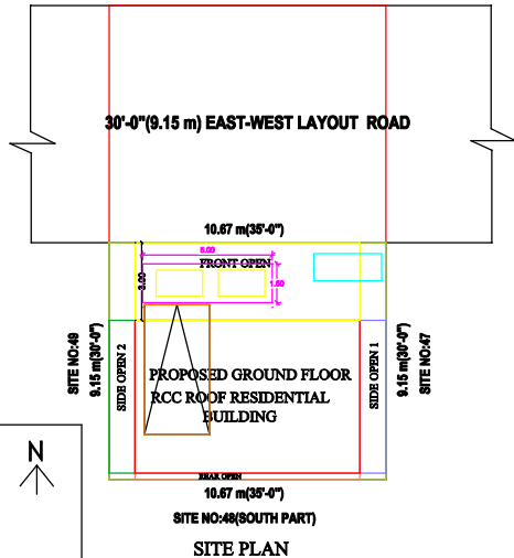
SITE PLAN
