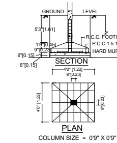
FOUNDATION DETAILS
