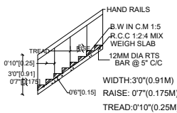
STAIR CASE DETAILS:-
