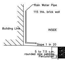
PERCOLATION PIT
