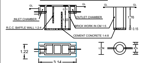
DETAILS OF SEPTIC TANK & SOAK PIT.
