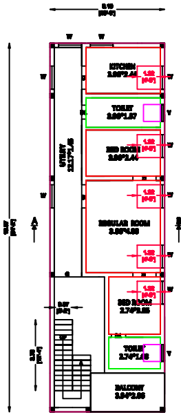
PROPOSED FIRST FLOOR BUILDING PLAN 1:100
