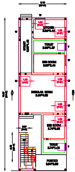
PROPOSED GROUND FLOOR BUILDING PLAN 1:100
