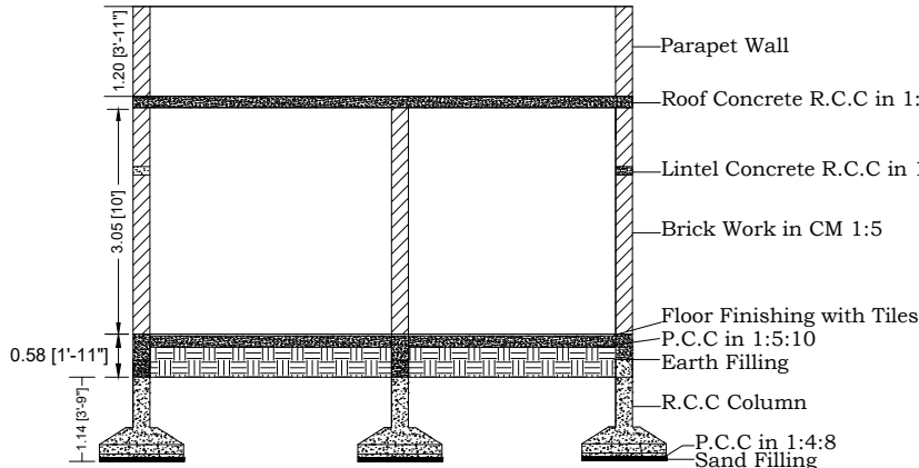
SECTION X-X
