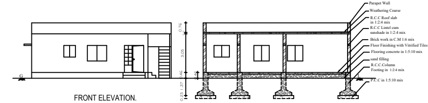
SECTION "A-B"
