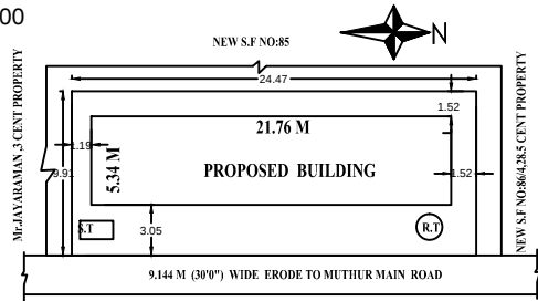
SITE PLAN SCALE = 1 : 500
