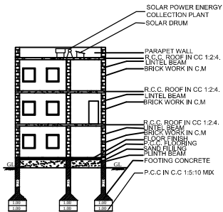
SECTION ON AB, CD & EF
