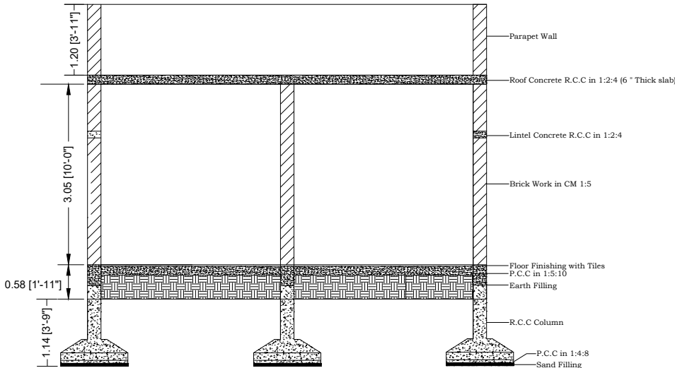
SECTION X-X
