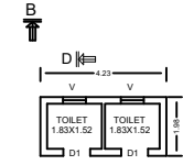
GROUND FLOOR PLAN (TOILET BLOCK) SCALE 1:100
