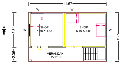
GROUND FLOOR PLAN (BLOCK 1) SCALE 1:100
