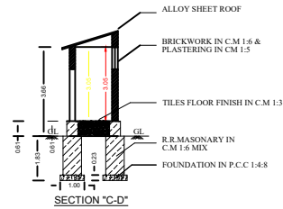
SECTION "C-D"
