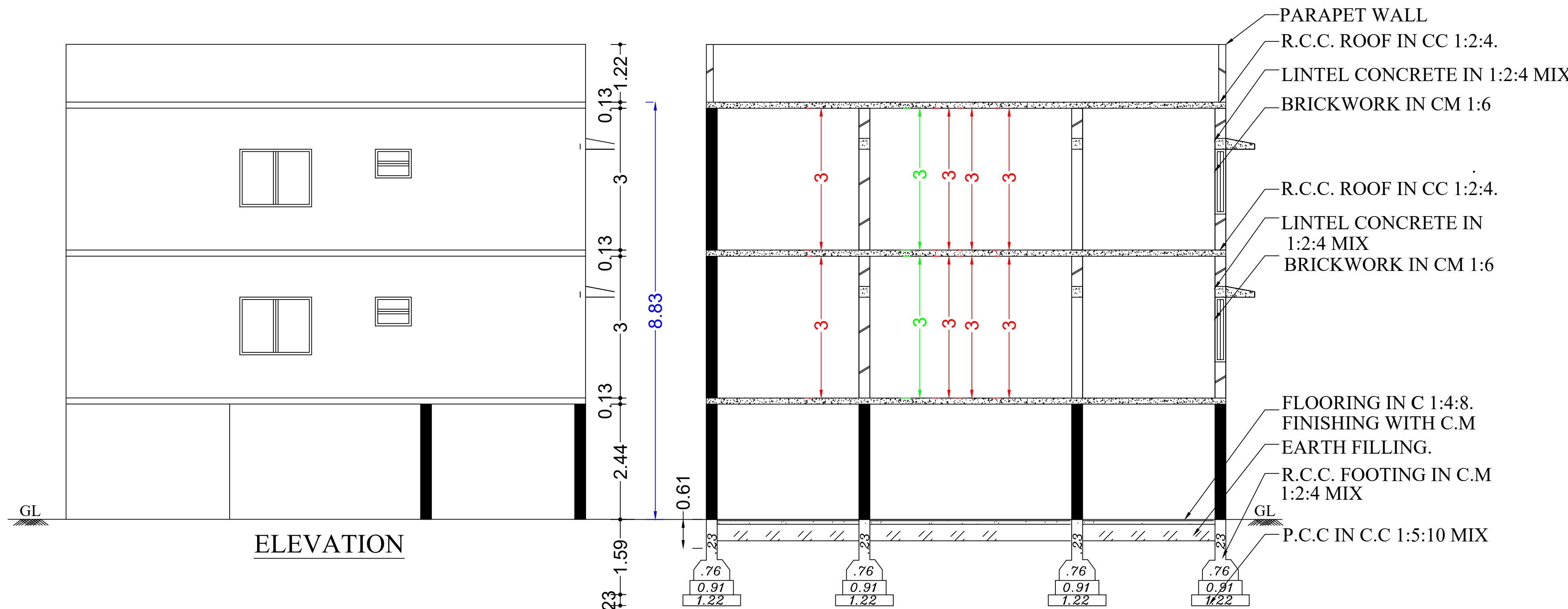
SECTION ON HK'
