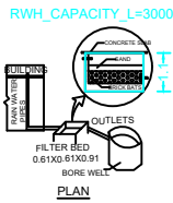
RAIN WATER HARVESTING SUMP
