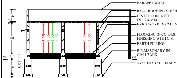
SECTION HK'
