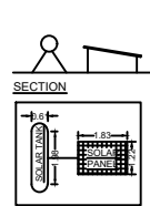
SOLAR SYSTEM
