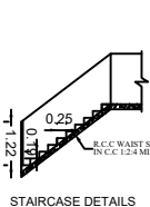
STAIRCASE DETAILS
