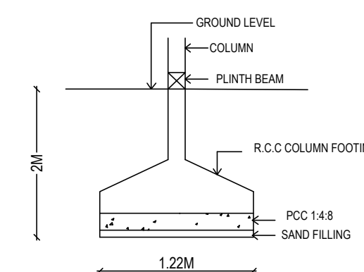
COLUMN FOOTING SECTION
