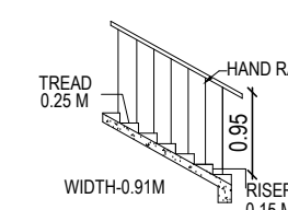
STAIRCASE DETAILS
