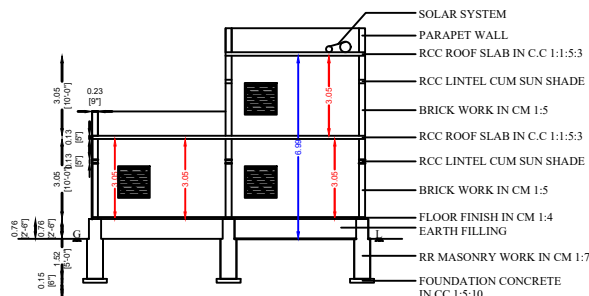
SECTION "AA","BB"
