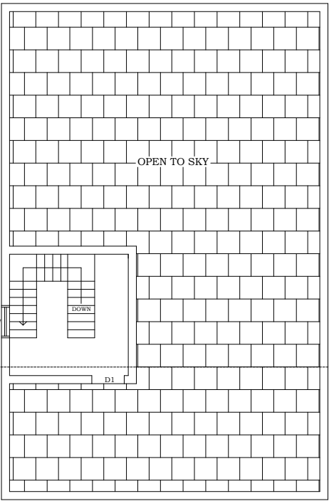
TERRACE FLOOR
