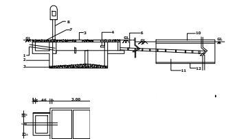
septic tank SEPTIC TANK
