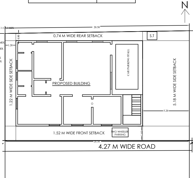
DETAILED SITE PLAN SCALE 1:100
