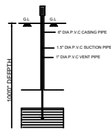
SECTION ON - "AB"
