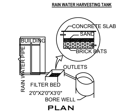
RAIN WATER HARVESTING TANK PLAN
