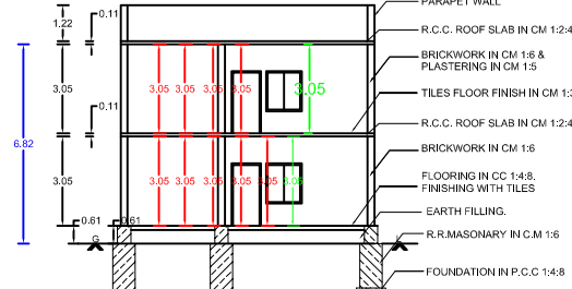
SECTION "A-B"
