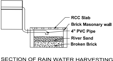
SECTION OF RAIN WATER HARVESTING
