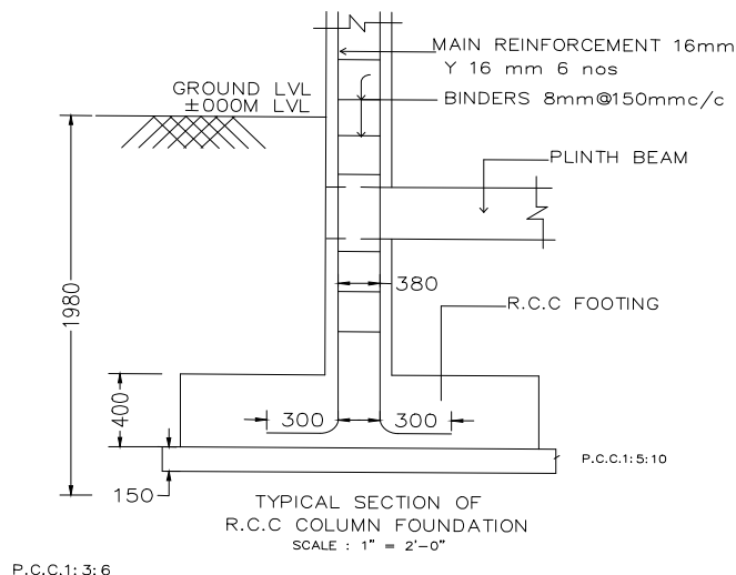
TYPICAL SECTION OF R.C.C COLUMN FOUNDATION
