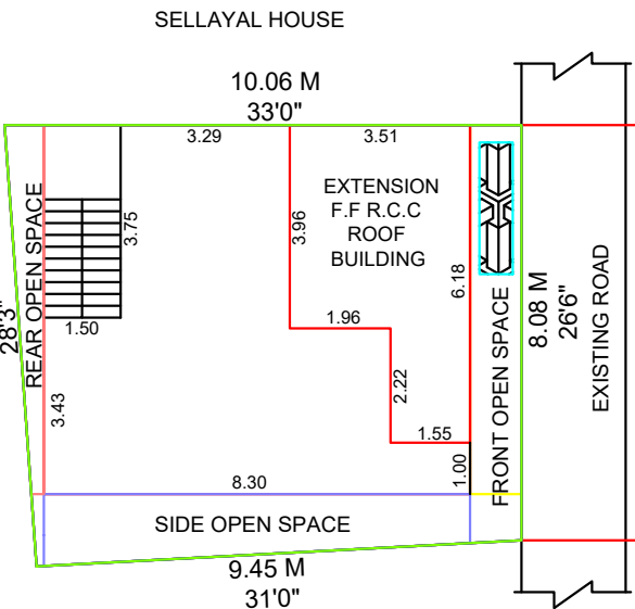
SITE PLAN SCALE 1CM :1M
