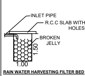
RAIN WATER HARVESTING FILTER BED
