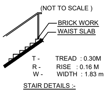
STAIR DETAILS :-
