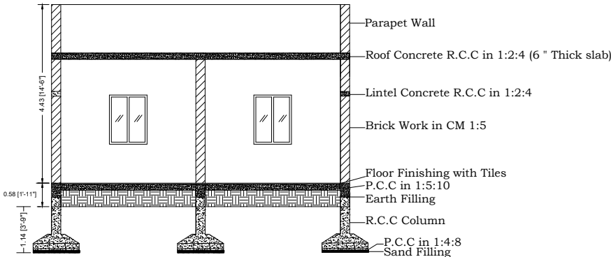
SECTION X-X
