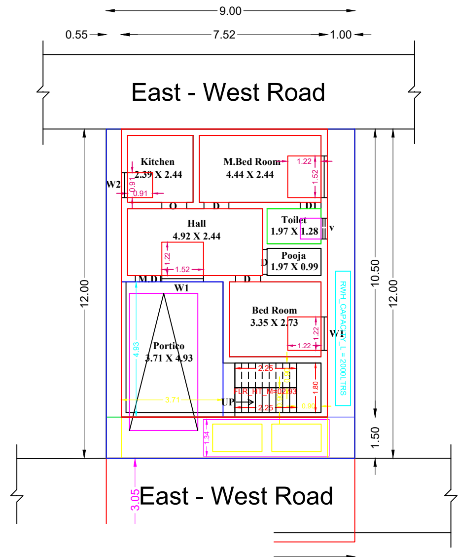
OR PLAN
