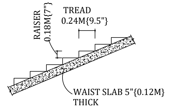
STAIRCASE DETAILS
