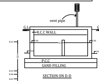
SECTION 0
