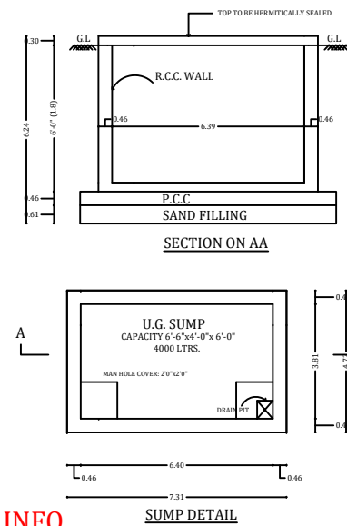
SCALE 1"=4'0"
