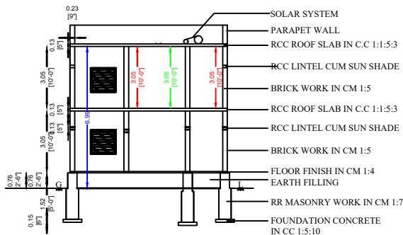
SECTION "AA","BB"
