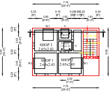
GROUND FLOOR PLAN (EXISTING BUILDING)
