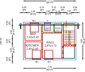
FIRST FLOOR PLAN (PROPOSED BUILDING)
