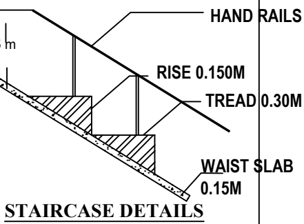
STAIRCASE DETAILS
