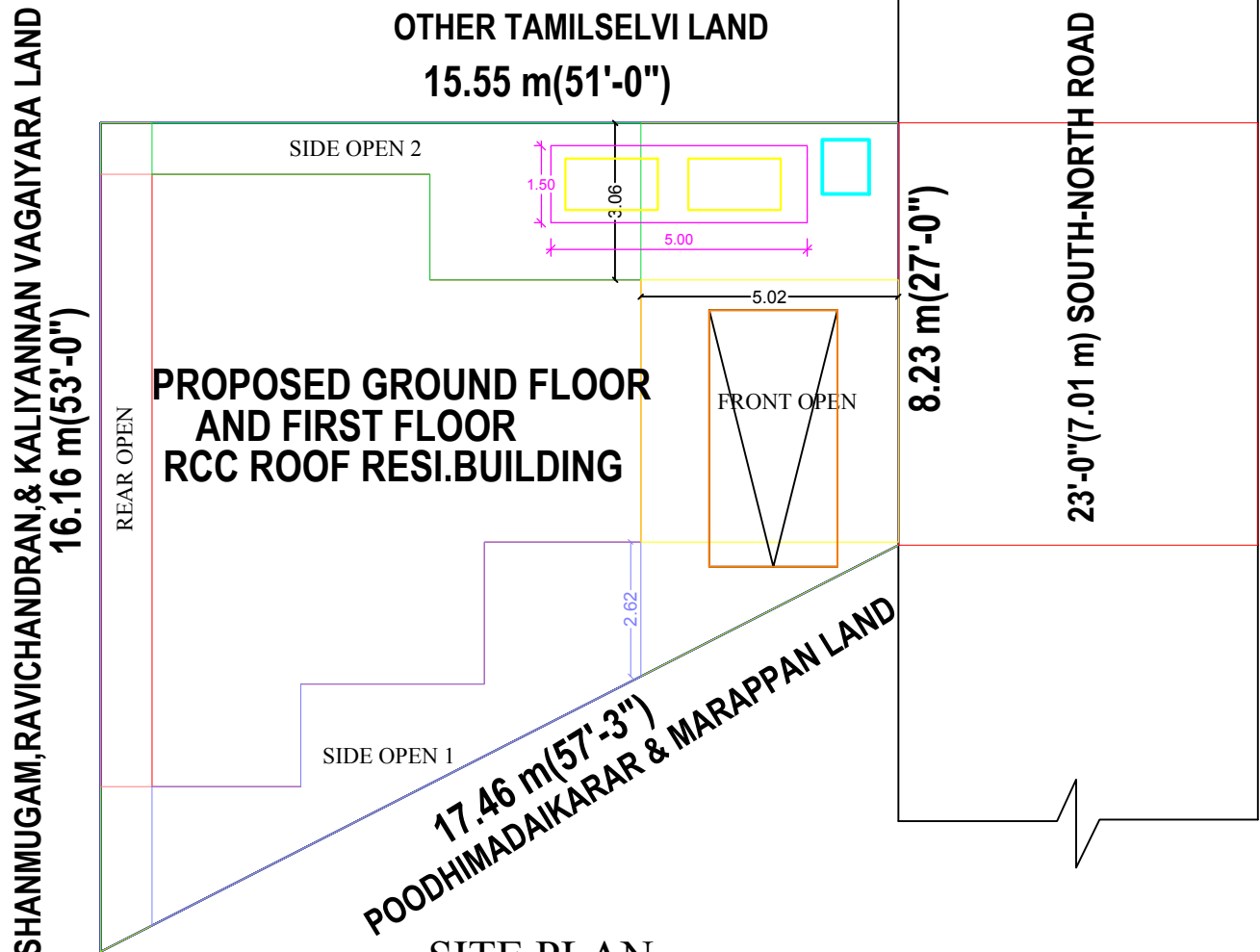
SITE PLAN
