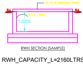
RWH_CAPACITY_L=2160LTRS
