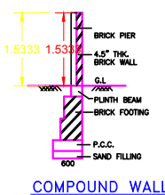
COMPOUND WALL
