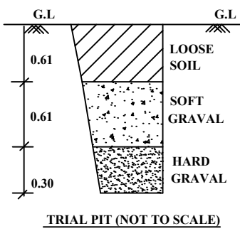
TRIAL PIT (NOT TO SCALE)
