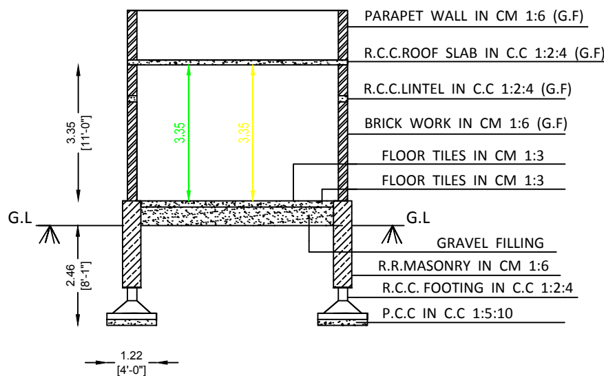
CROSS SECTION ON 'AB'
