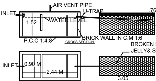
SEPTIC TANK (NOT TO SCALE)
