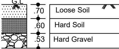
TRIAL PIT DETAILS (NOT TO SCALE)
