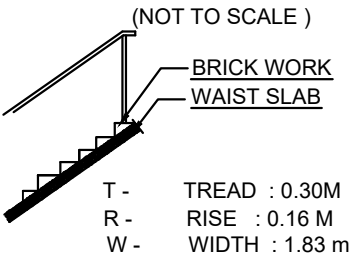
STAIR DETAILS :-
