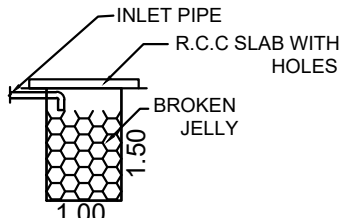
RAIN WATER HARVESTING FILTER BED
