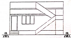
FRONT ELEVATION
