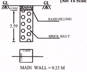
DETAILS OF RAINWATER HARVESTING TANK. (Not To Scale)
