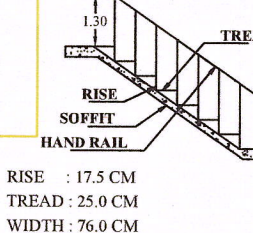
STAIRCASE DETAILS (Not To Scale)
