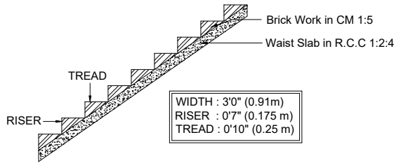
STAIRCASE DETAILS
