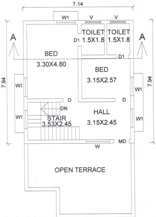
PLAN OF FIRST FLOOR
