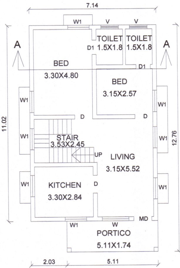
PLAN OF GROUND FLOOR
