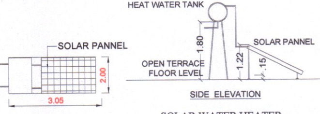
SOLAR WATER HEATER (NOT TO SCALE)
