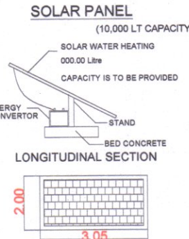
SOLAR PANEL (10,000 LT CAPACITY)
