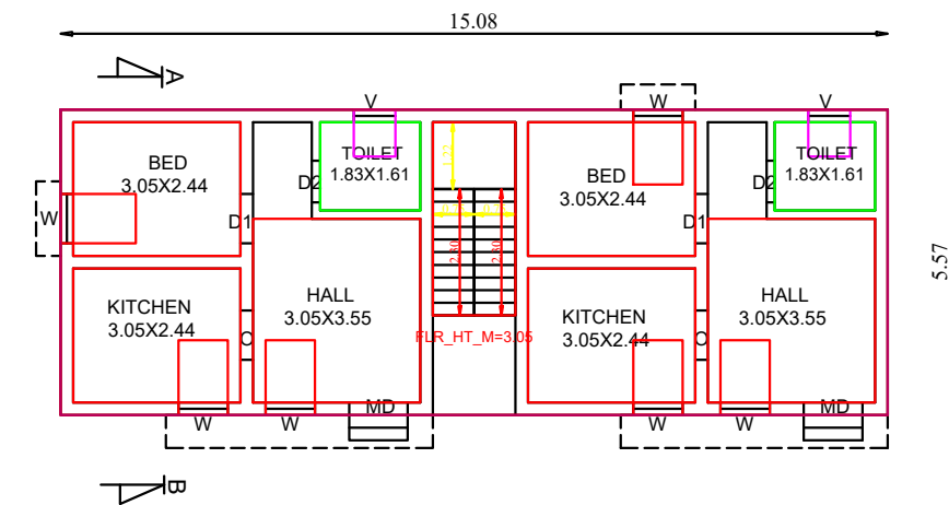
GROUND FLOOR PLAN SCALE 1 CM = 1 M
