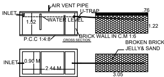
SEPTIC TANK (NOT TO SCALE)
