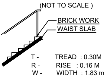
STAIR DETAILS :-
