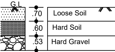
TRIAL PIT DETAILS (NOT TO SCALE)
