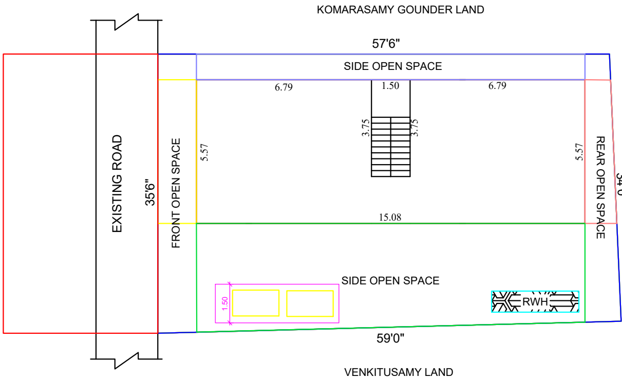
SITE PLAN SCALE 1CM:1M
