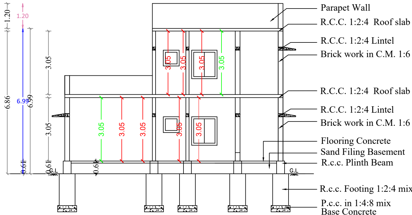
TYPICAL SECTION
