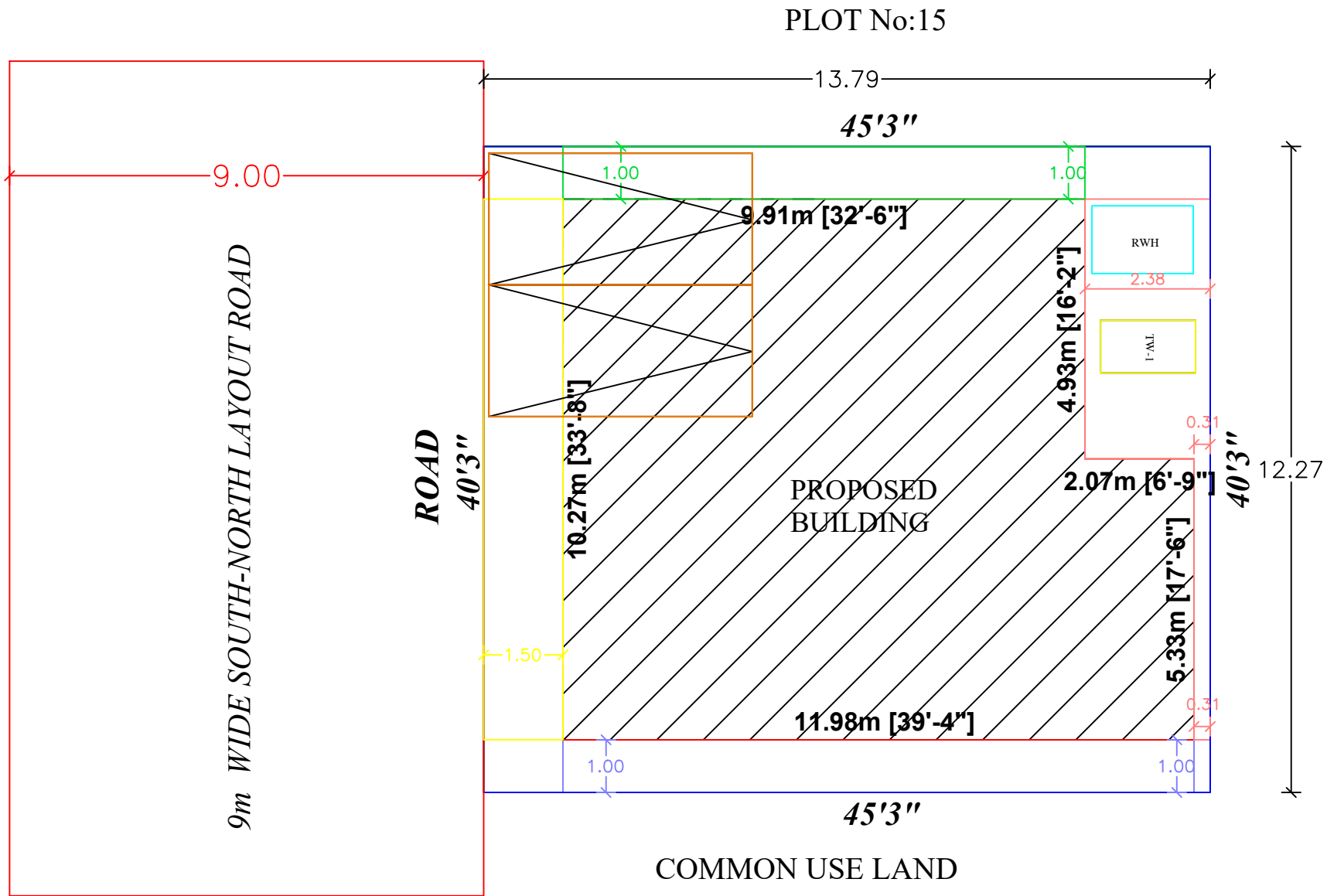
SITE PLAN
