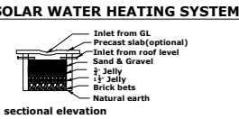
sectional elevation
