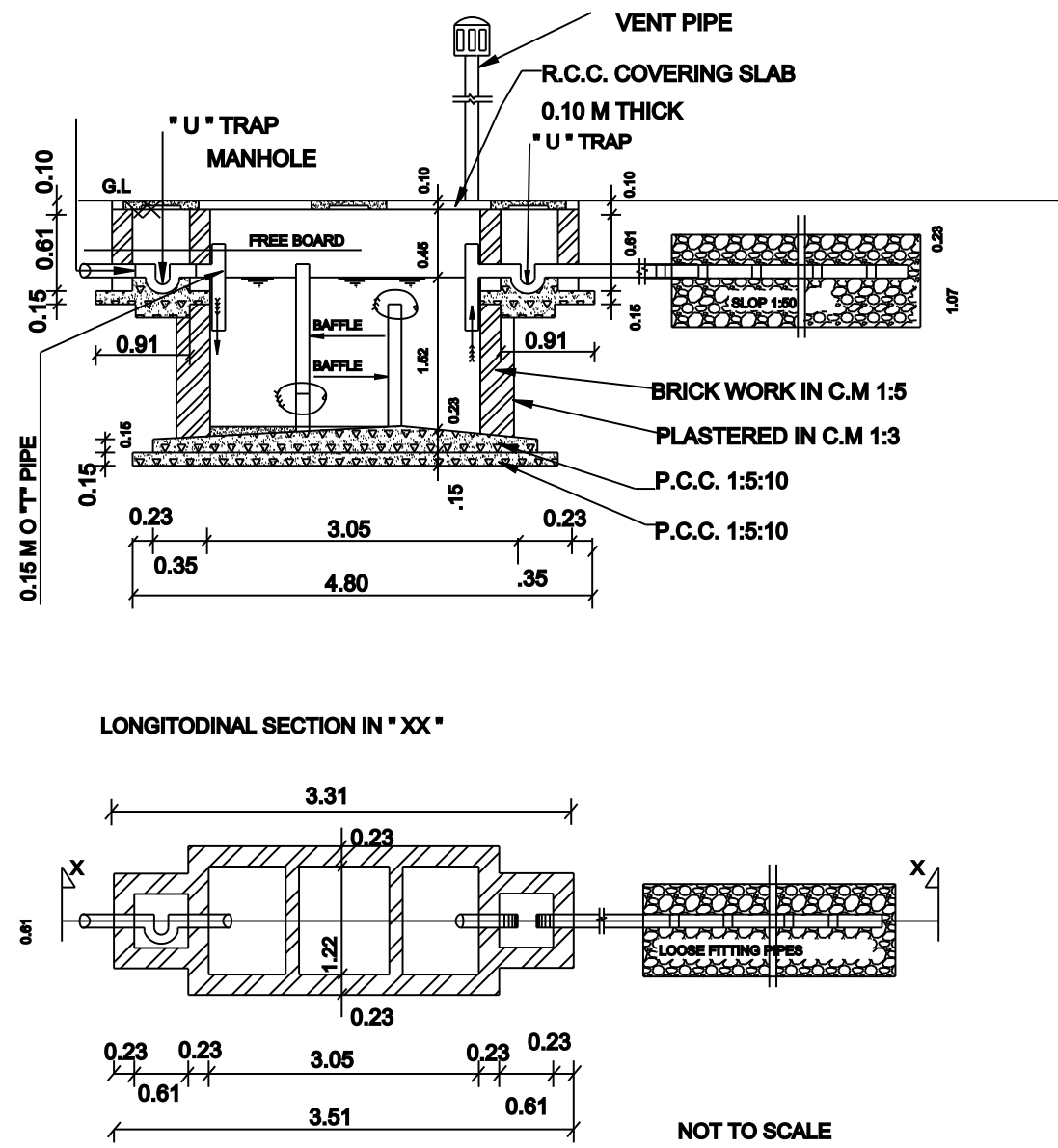
SEPTICK TANK & DISPERSION TRINCH
