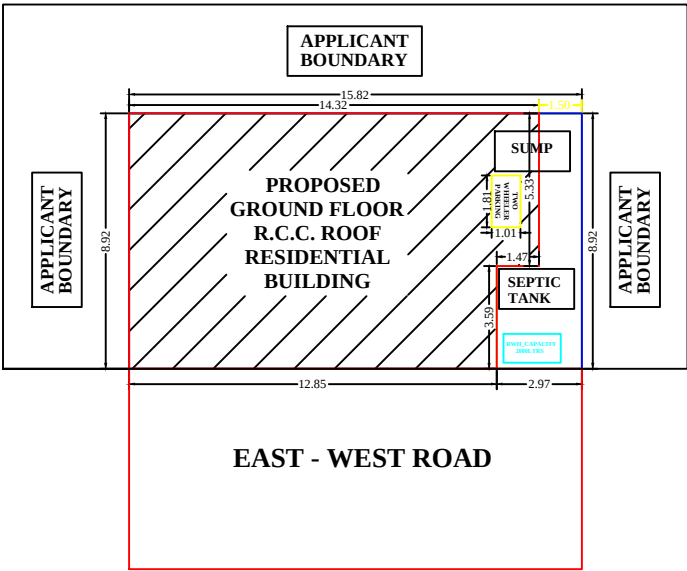
SITE PLAN
