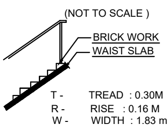
STAIR DETAILS :-
