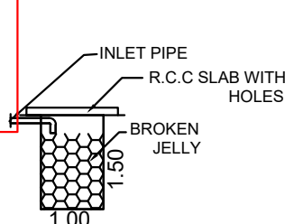
RAIN WATER HARVESTING FILTER BED
