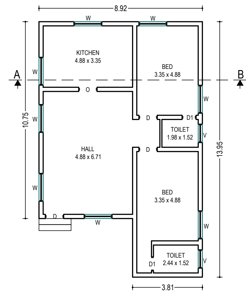
SITE / GROUND FLOOR PLAN
