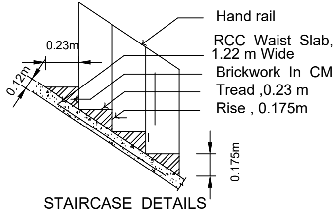
STAIRCASE DETAILS
