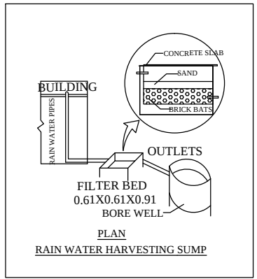
PLAN RAIN WATER HARVESTING SUMP
