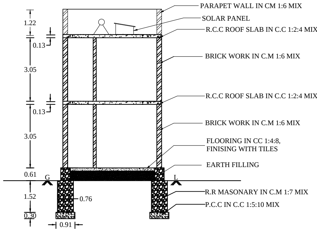
SECTION "A-B"
