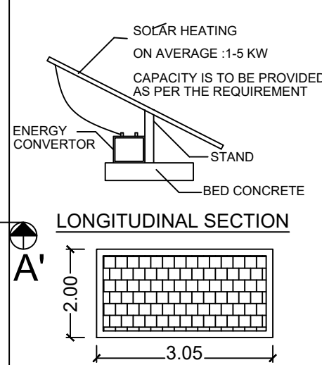
SOLAR SYSTEM:
