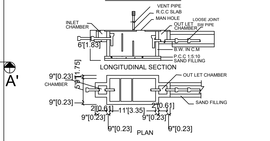
SEPTIC TANK:
