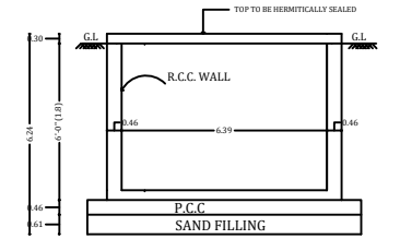
SECTION ON AA
