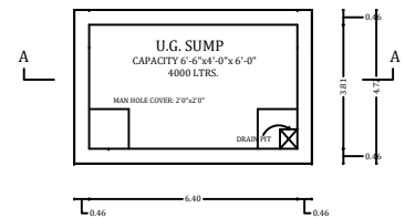
SUMP DETAIL
