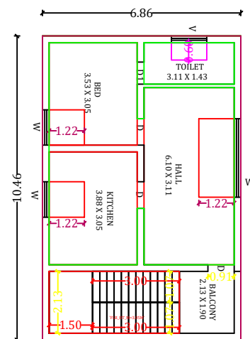
ADDITIONAL PROPOSED FIRST FLOOR PLAN
