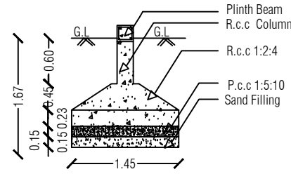
COLUMN FOOTING DETAILS
